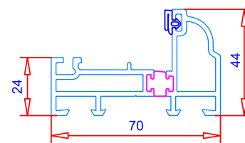
French Door Low Threshold
