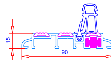
Part M Low Threshold
