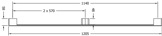
Front Profile
