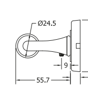
Side Profile
