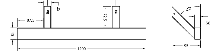
Side Profile
