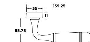
Top Profile
