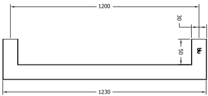
Side Profile
