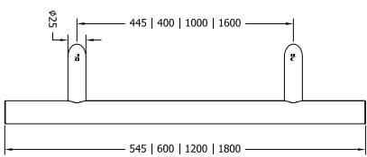
Side Profile
