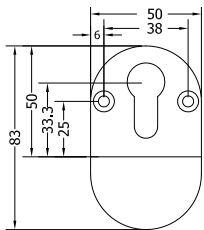
Front Profile
