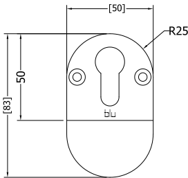
Front Profile
