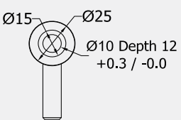
Rear Profile
