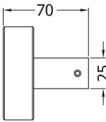
Side Profile
