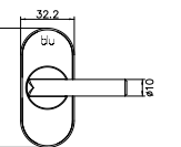
Side Profile
