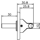
Top Profile
