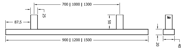
Side Profile
