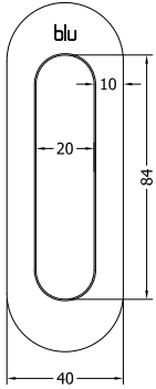
Front Profile
