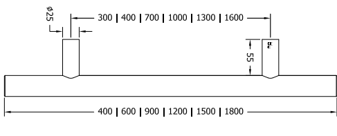
Side Profile
