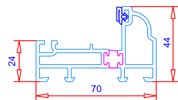
French Door Low Threshold
